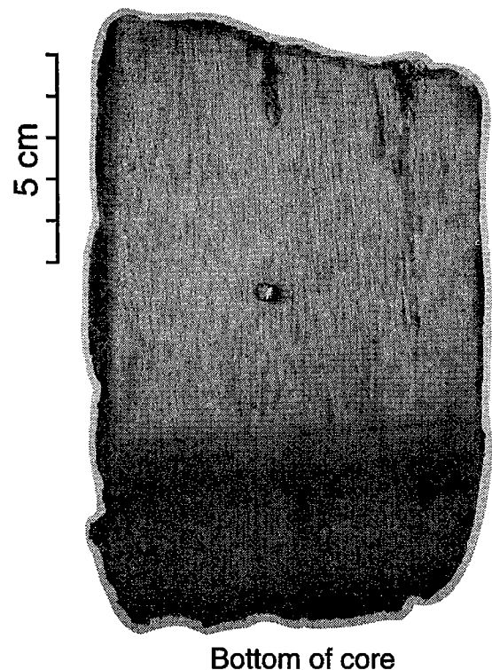
Fig. 5. Thick section of bottom section showing the darkening of the ice by ice algae (18 May 1997, site DYR). The hole in the center of the section was drilled to measure temperature inside the core.
